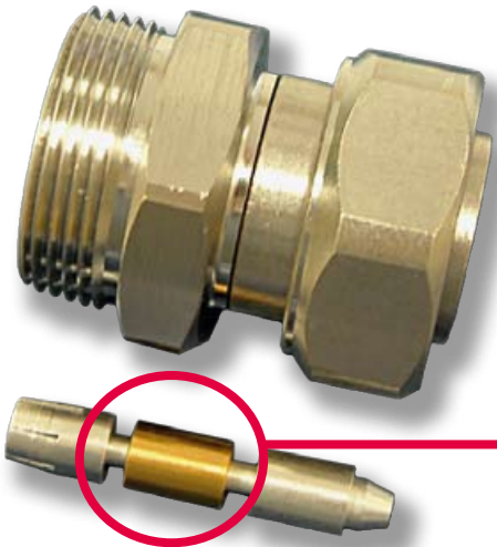
Test receptacle (male/female adaptor type 7-16)
